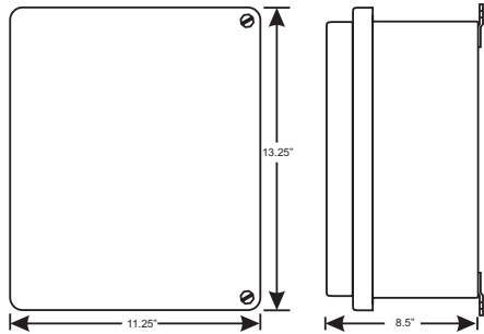
Fiberglass Enclosure (-FG Option)
