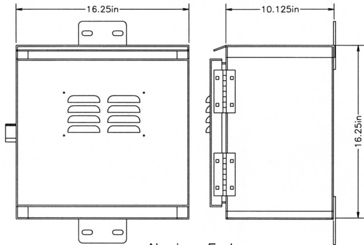
Aluminum Enclosure (-AL Option)
